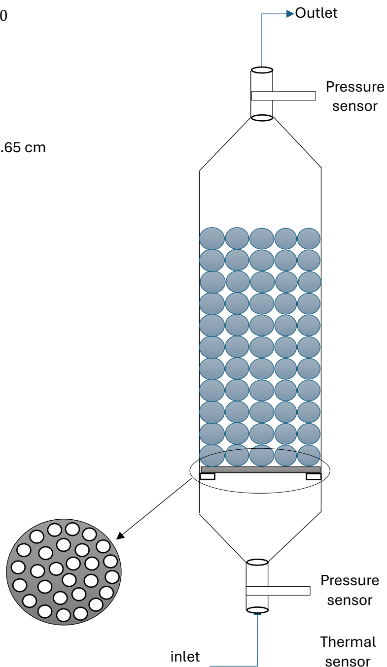
Single bed column
